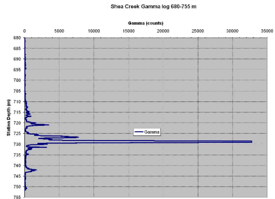
Figure 8: Shea Creek Test Gamma Log, 680 – 755 m
