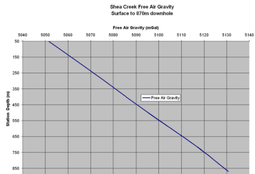
Figure 9: Shea Creek Gravity, Free Air Corrected
