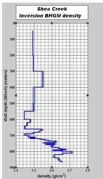
Figure 10: Shea Creek Test Bulk Density Log
