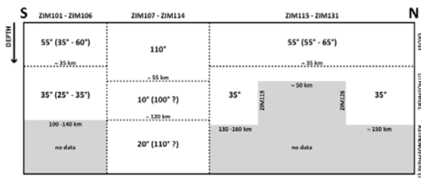
Figure 4. Sketch of the different strike directions for various parts of the ZIM line. In crustal depth a strike azimuth of 55° is dominant (strike ranges given in parentheses), but if analysed separately the sites above the Okavango dyke swarm indicate a strike direction parallel to the swarm orientation. In lithospheric depths a strike azimuth of 35° is the dominant direction.
